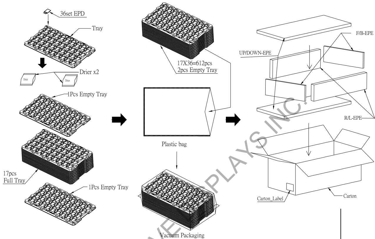
Figure 7-1 Packing Diagram
