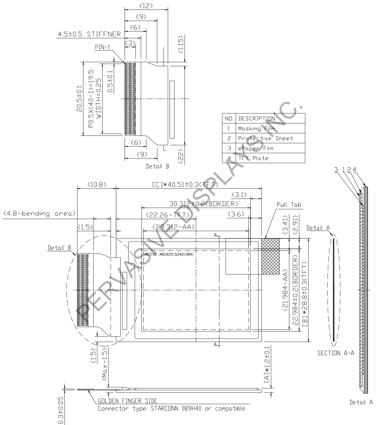
Figure 1-1 EPD Drawing
