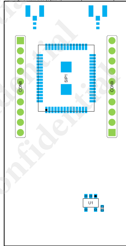
Bottom view
