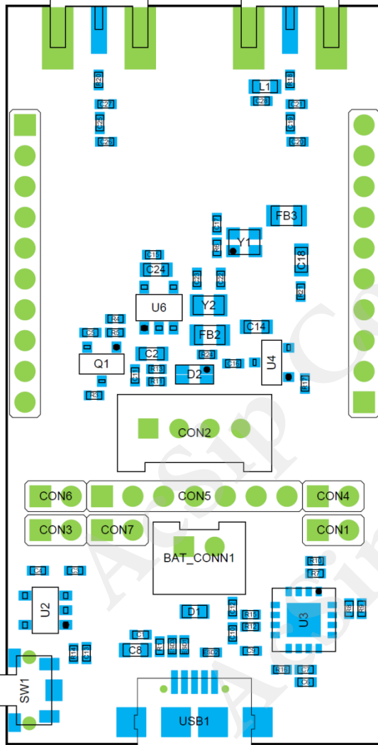
Top view
