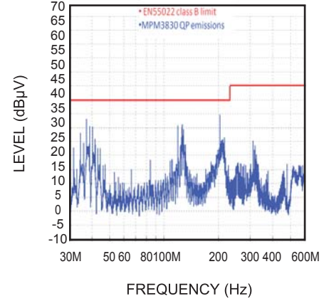
Radiated Emission
